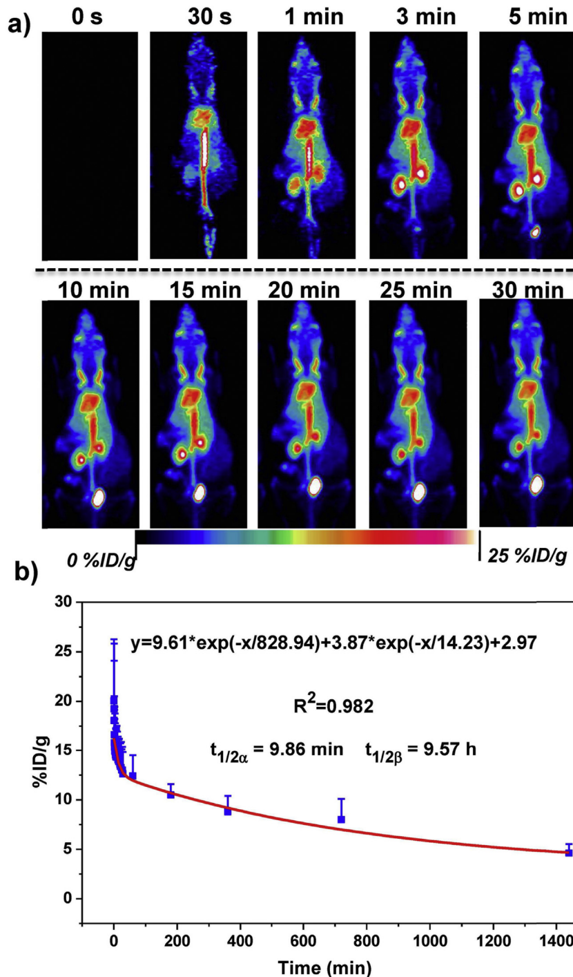
Fig. 2. a) Representative dynamic PET images of healthy mice after intravenous injection of ^{89}\text{Zr} -POM clusters within different time points. b) Time-activity curves of ^{89}\text{Zr} -POM in the blood ( n = 4 , mean \pm s.d.).
