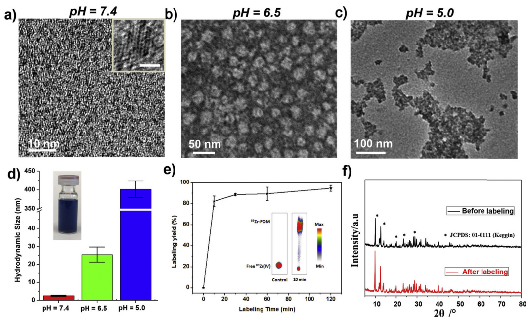
Fig. 1. Synthesis and characterization of 89 Zr-POM clusters. a–c) TEM images of POM clusters at pH = 7.4, 6.5, and 5.0. Insert in a) shows the High-resolution TEM image of one POM, scale bar: 1 nm. d) DLS measurements of POM clusters with successive acidifications from pH = 7.4 to pH = 6.5 and to pH = 5.0 (inset: photograph of the clusters dispersed in water). e) Time-dependent 89 Zr-labeling yield in HEPES buffer solution with POM clusters. Inset: the autoradiographic image of TLC plates of 89 Zr-POM clusters acquired at 37 °C using PBS (pH = 5) as the developing solvent. Free 89 Zr(IV) was used as a control. f) Powder X-ray diffraction (XRD) of POM nanoclusters before and after radiolabeling with 89 Zr.
